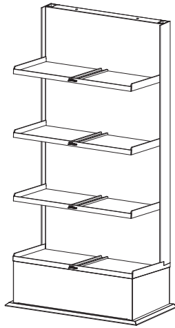
UPPER SECTION (x1)
